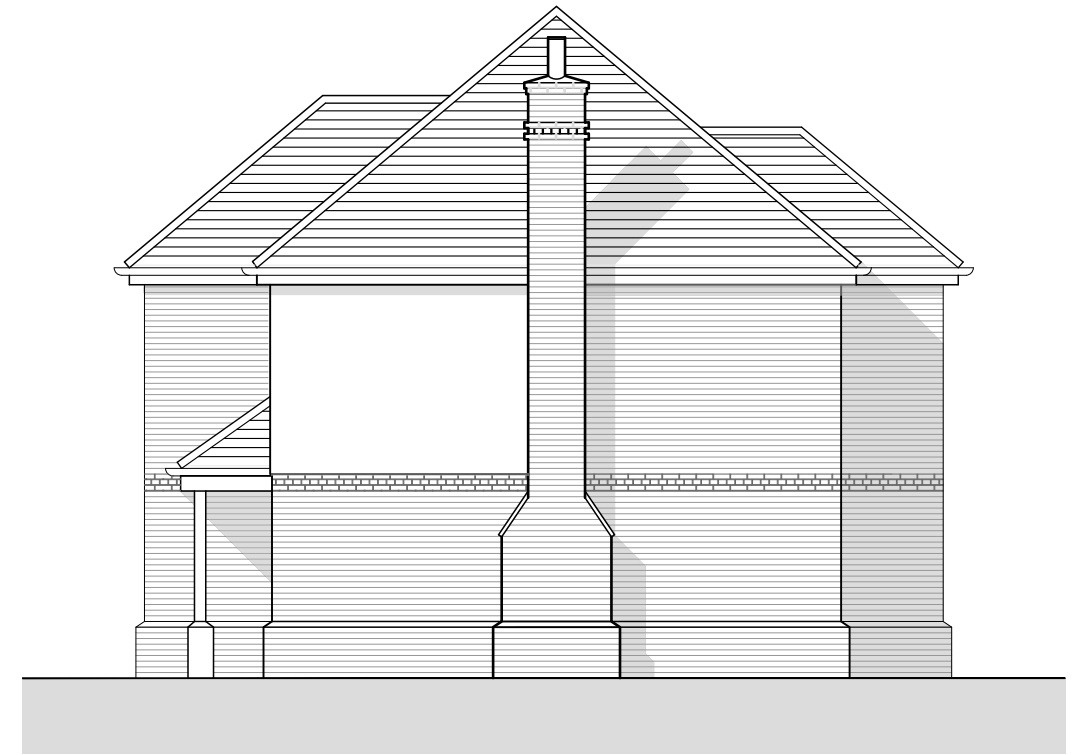
SIDE ELEVATION
